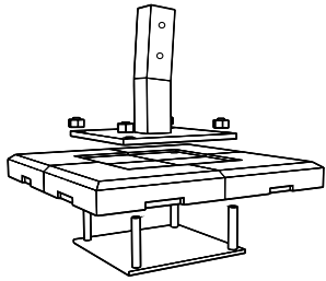
Large concrete base Grande base in cemento Velika cementna baza (250-500-750 kg)
